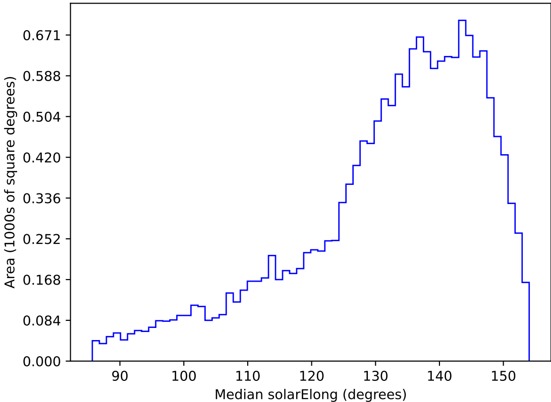
ddf_acor_sf10_lsf30_lsr10_v3.4_10yrs WFD u band: Median solarElong
