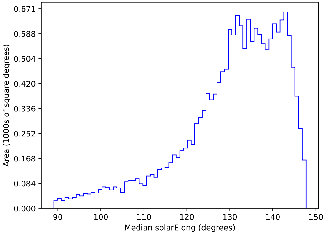
ddf_acor_sf10_lsf30_lsr10_v3.4_10yrs WFD r band: Median solarElong
