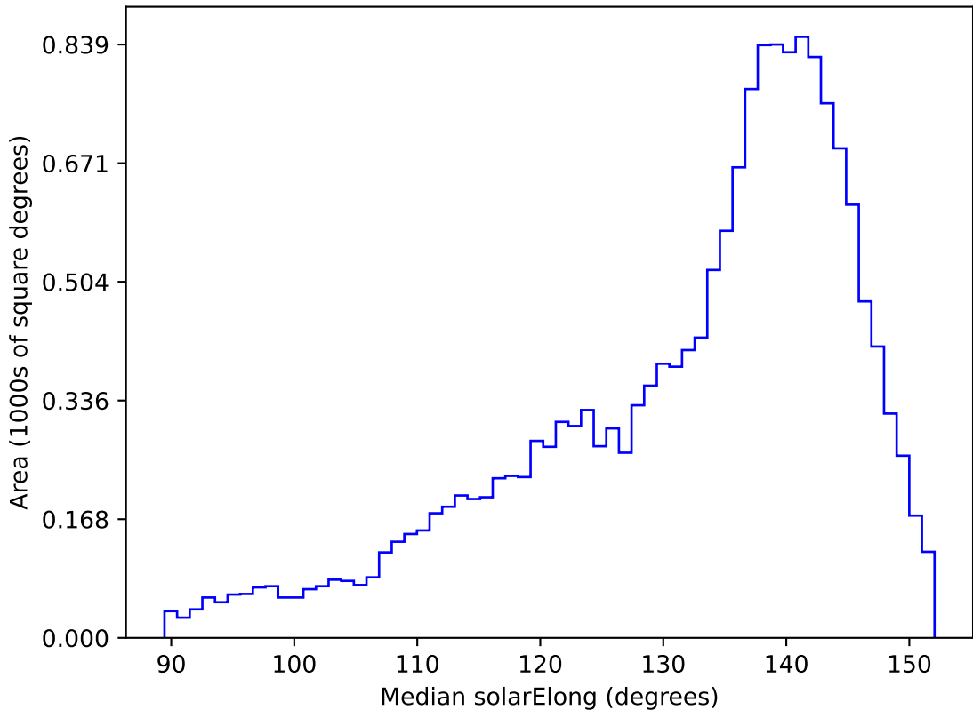
ddf_acor_sf10_lsf30_lsr10_v3.4_10yrs WFD g band: Median solarElong
