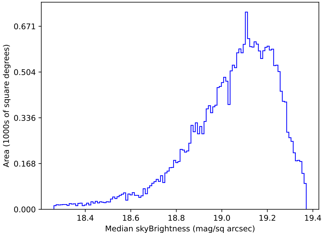
ddf_acor_sf10_lsf30_lsr10_v3.4_10yrs Yr 1 z band: Median skyBrightness
