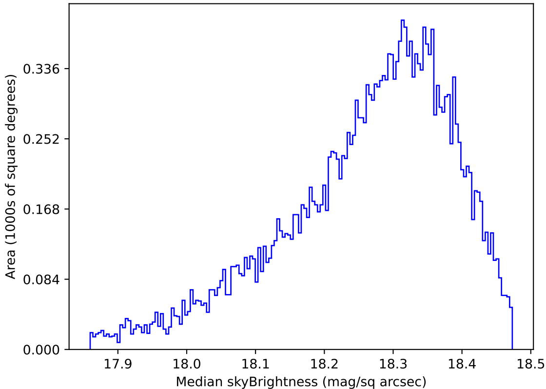
ddf_acor_sf10_lsf30_lsr10_v3.4_10yrs Yr 1 y band: Median skyBrightness
