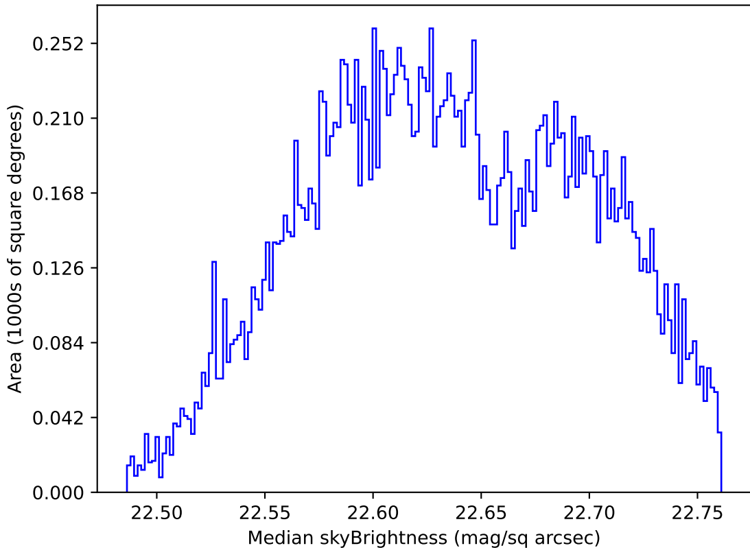
ddf_acor_sf10_lsf30_lsr10_v3.4_10yrs Yr 1 u band: Median skyBrightness
