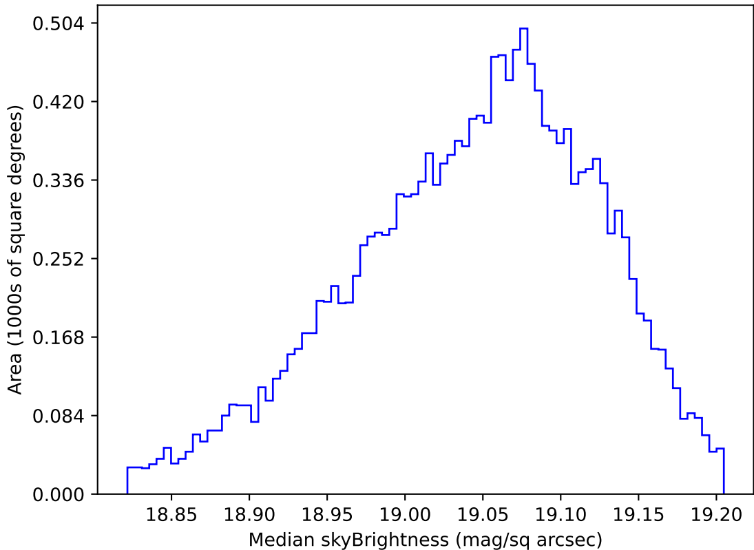
ddf_acor_sf10_lsf30_lsr10_v3.4_10yrs WFD z band: Median skyBrightness
