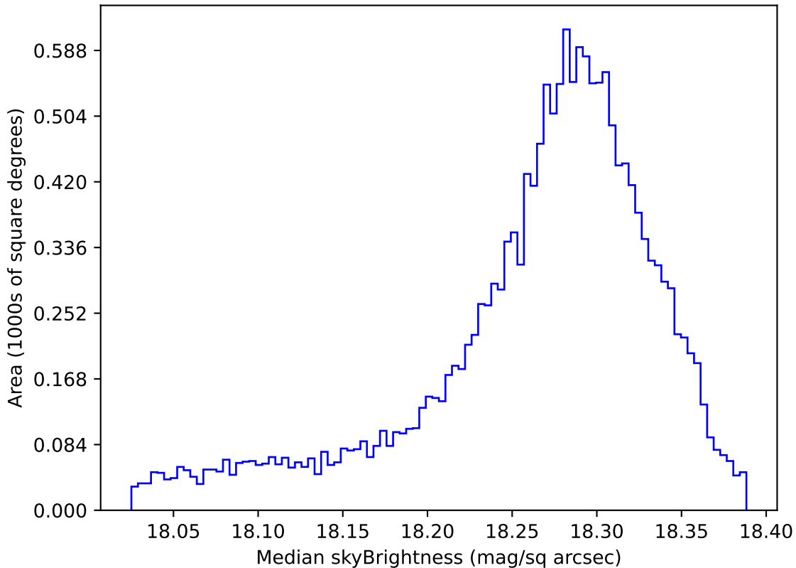
ddf_acor_sf10_lsf30_lsr10_v3.4_10yrs WFD y band: Median skyBrightness
