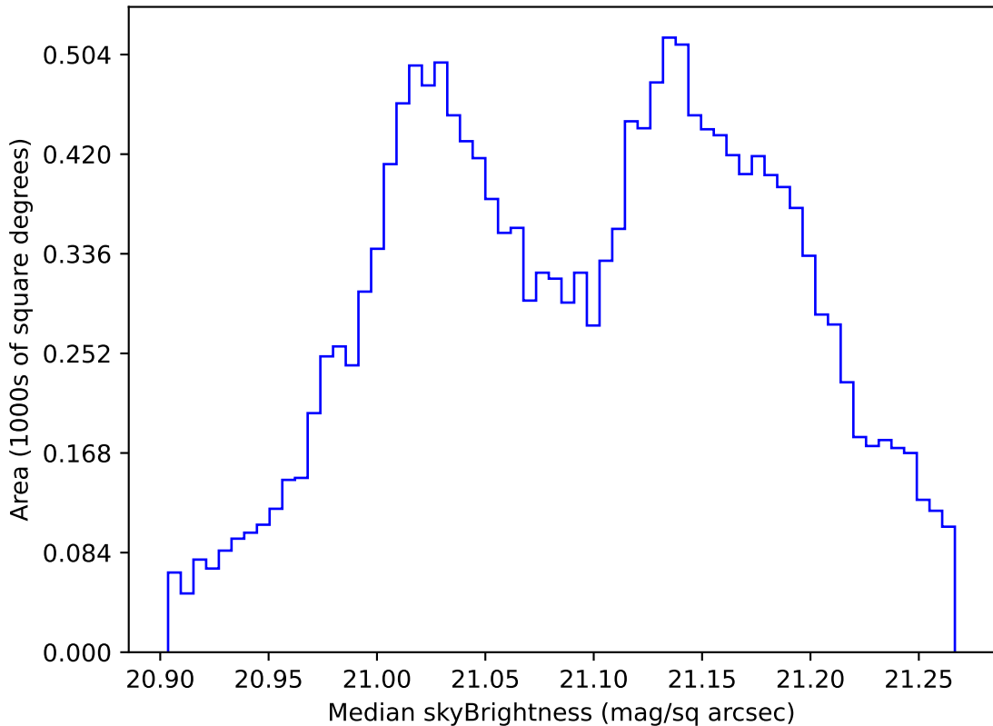
ddf_acor_sf10_lsf30_lsr10_v3.4_10yrs WFD r band: Median skyBrightness
