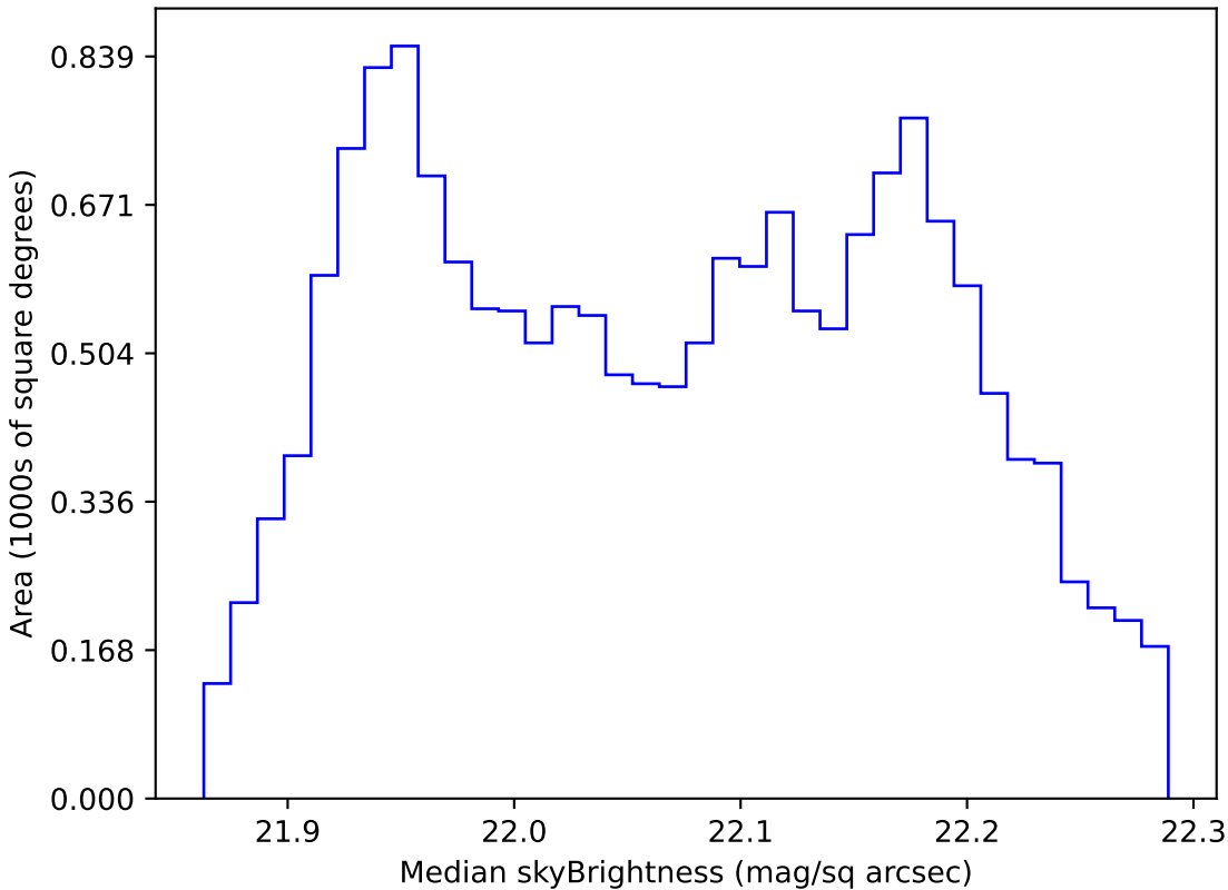
ddf_acor_sf10_lsf30_lsr10_v3.4_10yrs WFD g band: Median skyBrightness
