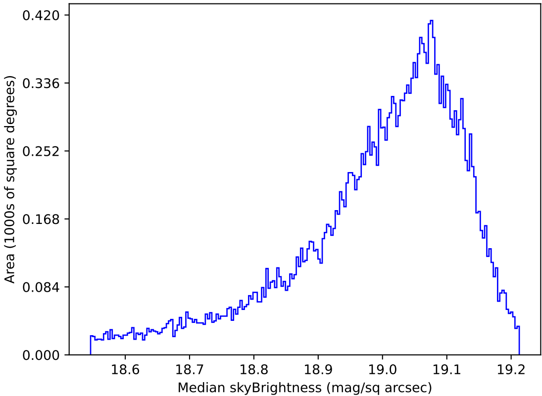
ddf_acor_sf10_lsf30_lsr10_v3.4_10yrs All sky z band: Median skyBrightness
