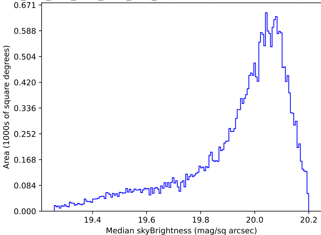
ddf_acor_sf10_lsf30_lsr10_v3.4_10yrs All sky i band: Median skyBrightness
