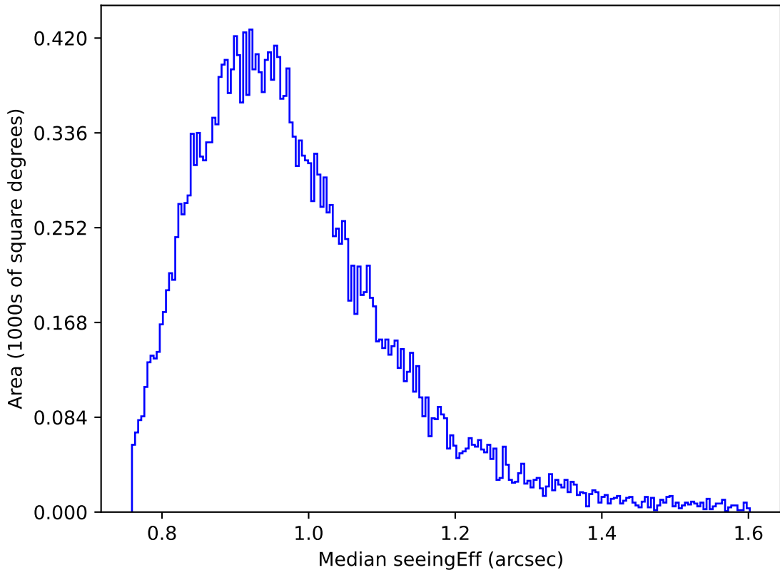
ddf_acor_sf10_lsf30_lsr10_v3.4_10yrs Yr 1 z band: Median seeingEff
