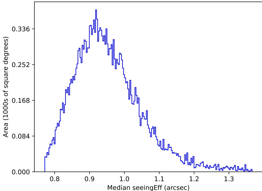
ddf_acor_sf10_lsf30_lsr10_v3.4_10yrs Yr 1 y band: Median seeingEff
