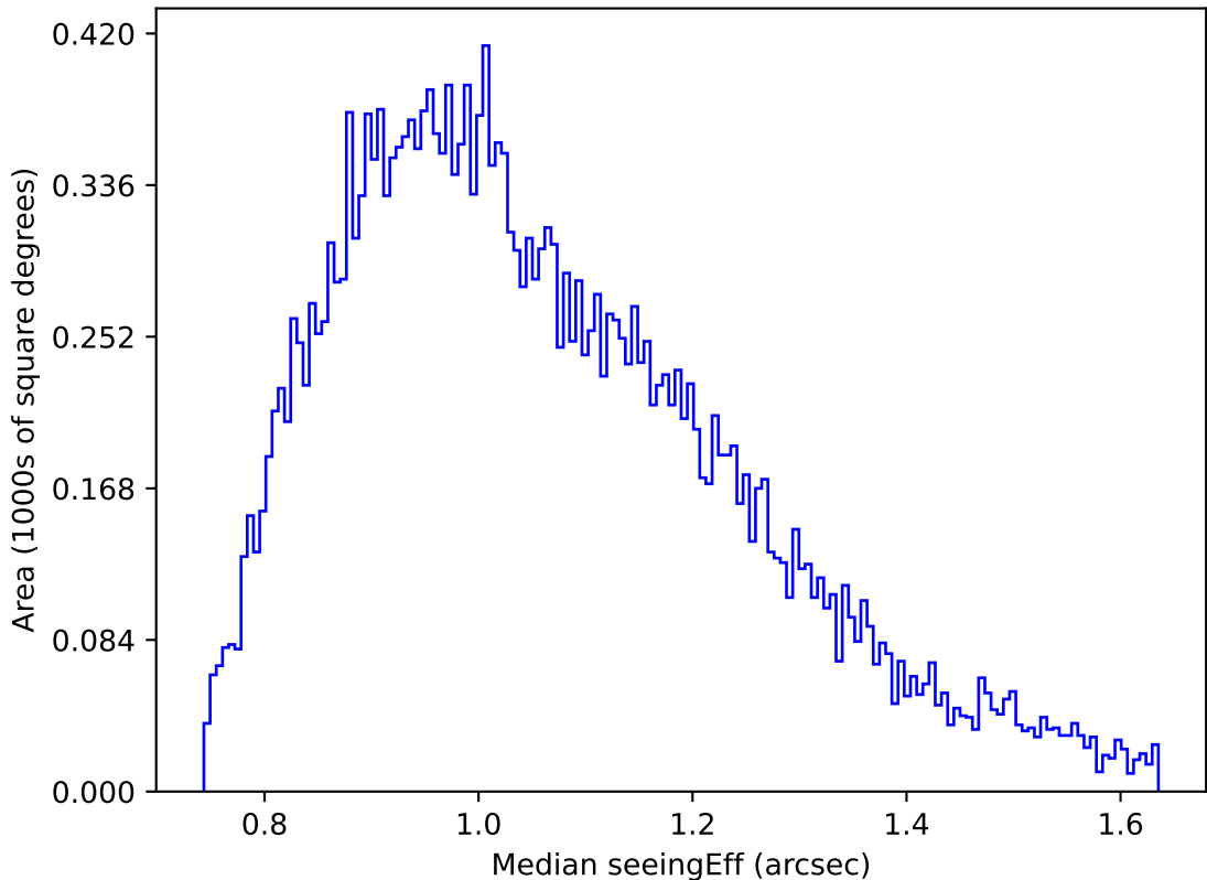
ddf_acor_sf10_lsf30_lsr10_v3.4_10yrs Yr 1 g band: Median seeingEff
