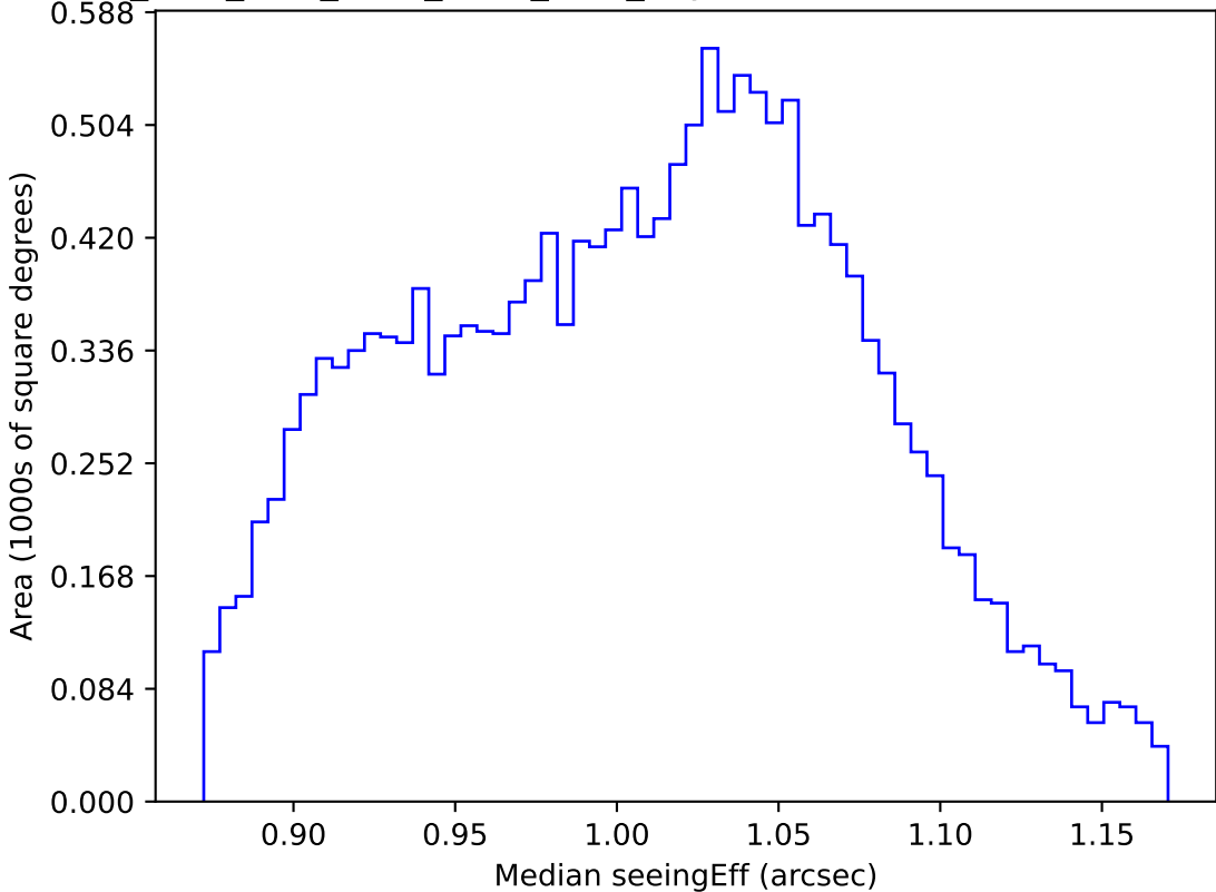
ddf_acor_sf10_lsf30_lsr10_v3.4_10yrs WFD z band: Median seeingEff
