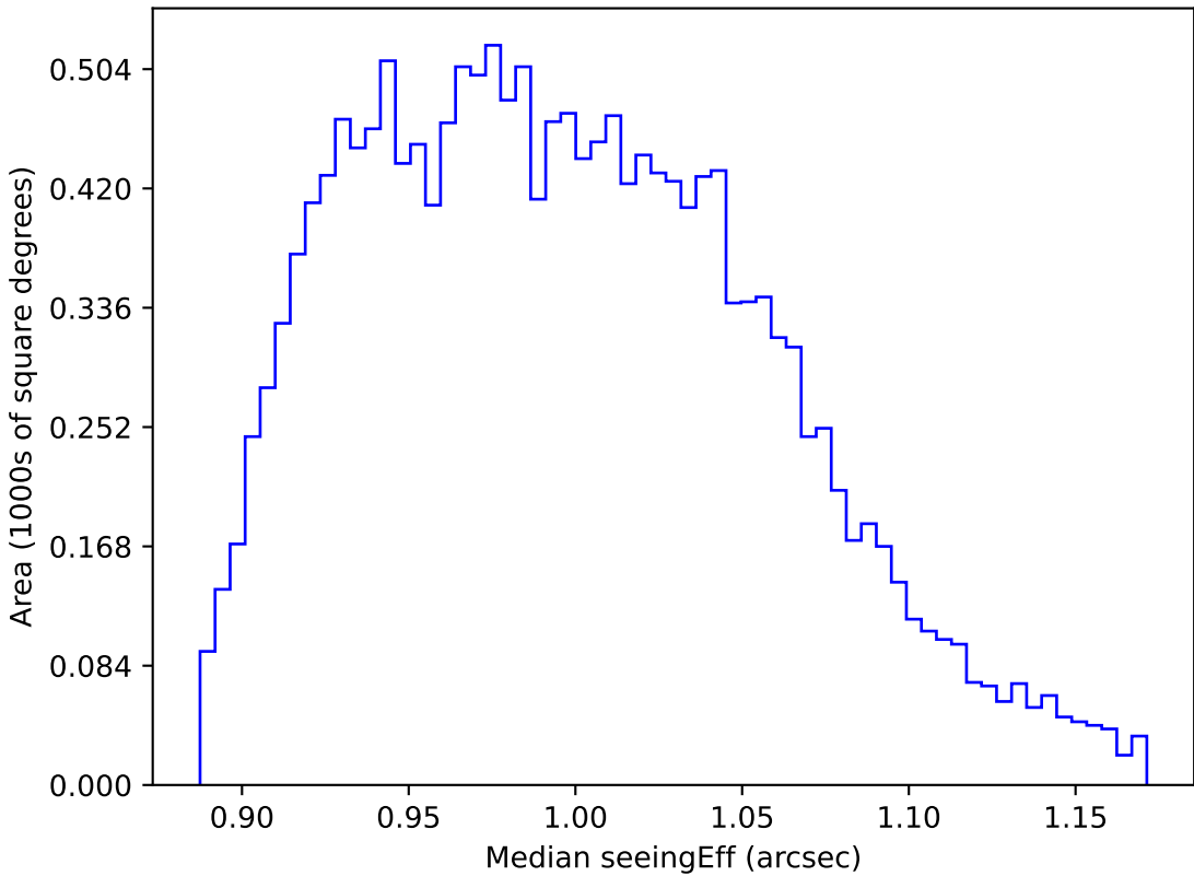
ddf_acor_sf10_lsf30_lsr10_v3.4_10yrs WFD y band: Median seeingEff
