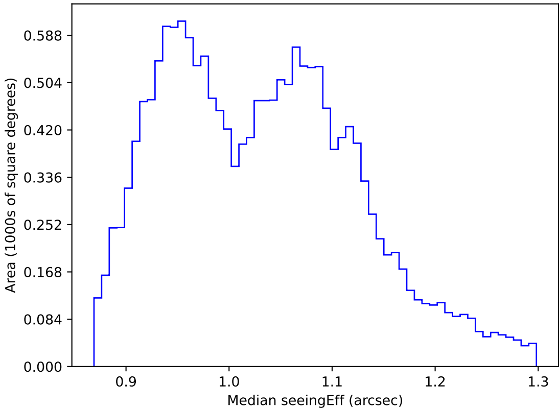
ddf_acor_sf10_lsf30_lsr10_v3.4_10yrs WFD r band: Median seeingEff
