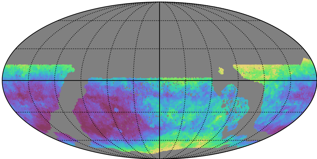
ddf_acor_sf10_lsf30_lsr10_v3.4_10yrs WFD i band: Median seeingEff
