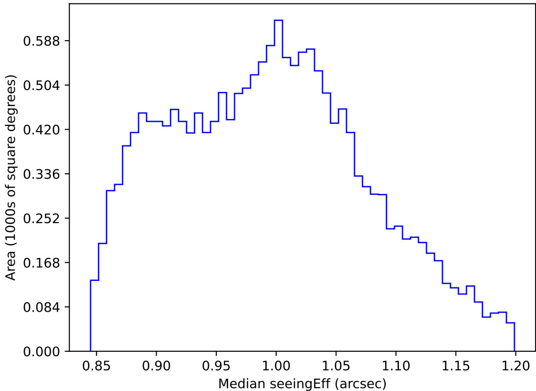
ddf_acor_sf10_lsf30_lsr10_v3.4_10yrs WFD i band: Median seeingEff
