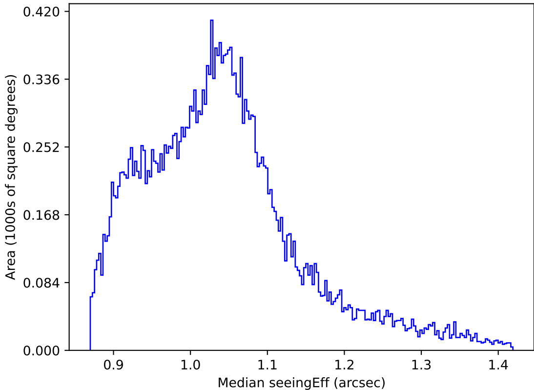
ddf_acor_sf10_lsf30_lsr10_v3.4_10yrs All sky z band: Median seeingEff
