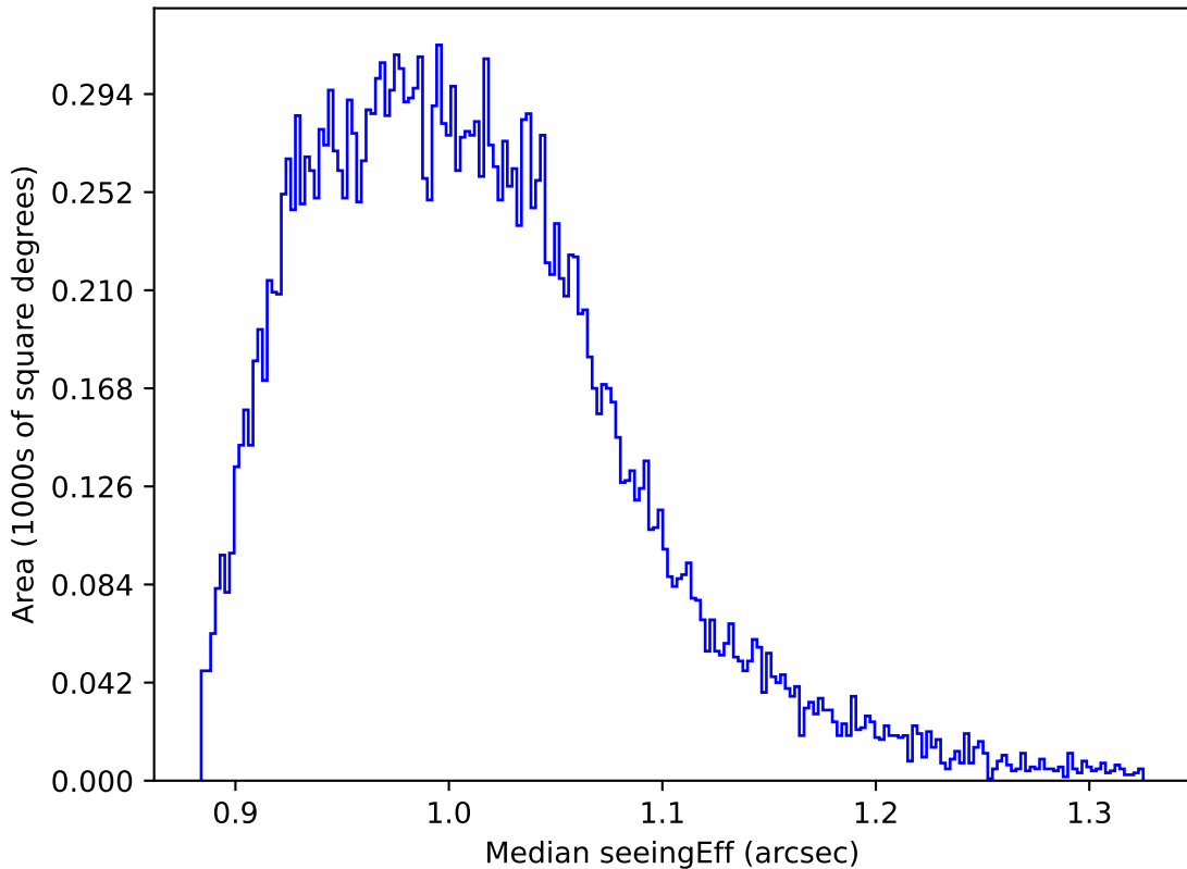
ddf_acor_sf10_lsf30_lsr10_v3.4_10yrs All sky y band: Median seeingEff
