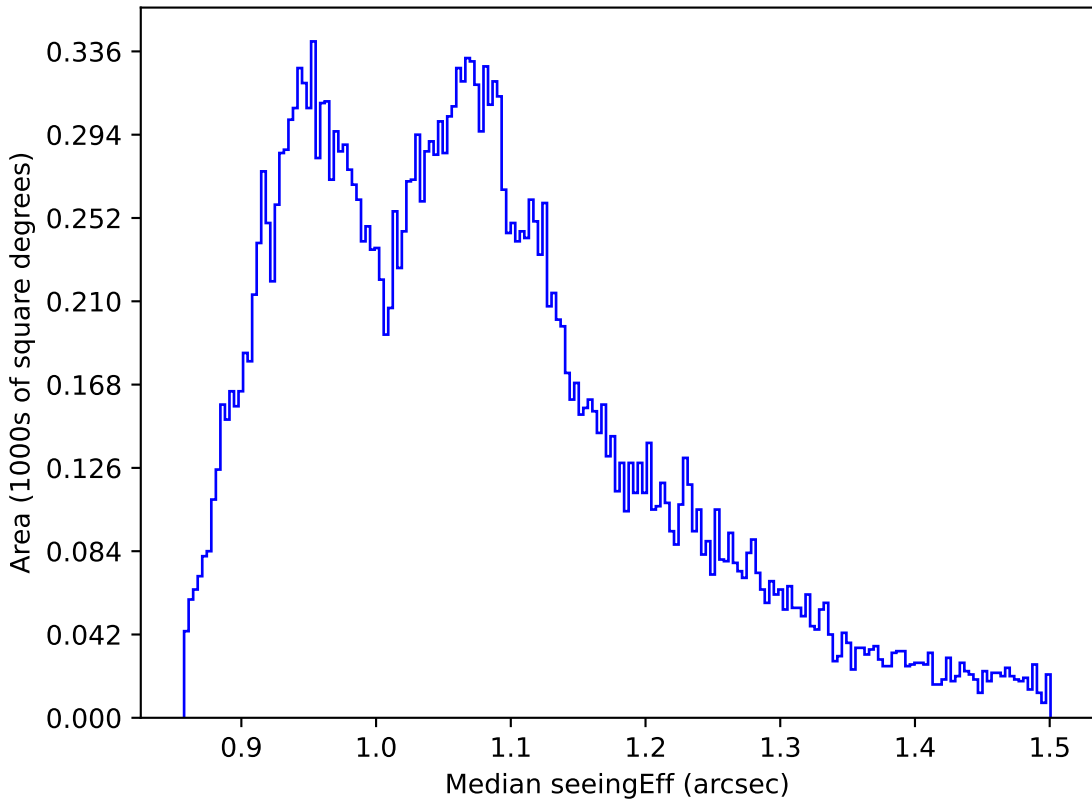
ddf_acor_sf10_lsf30_lsr10_v3.4_10yrs All sky r band: Median seeingEff
