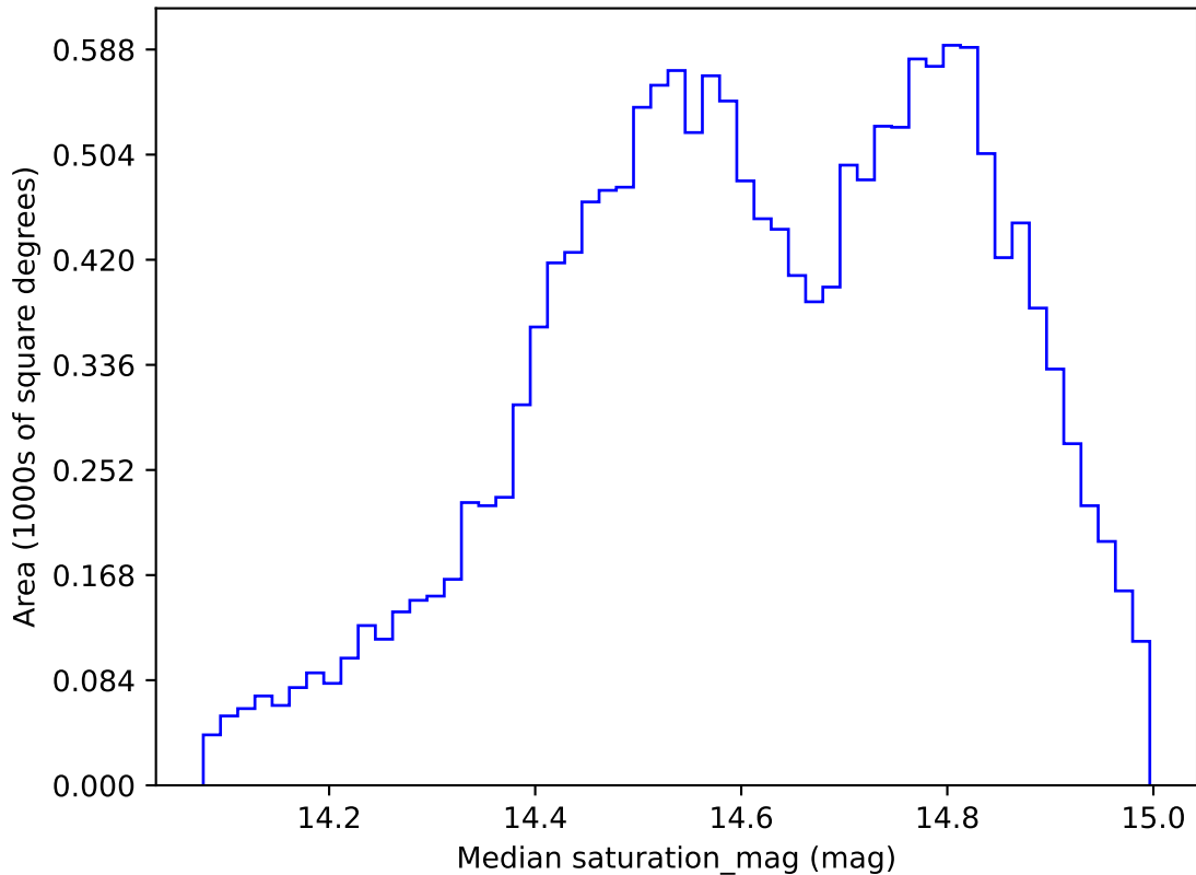
ddf_acor_sf10_lsf30_lsr10_v3.4_10yrs WFD r band: Median saturation_mag
