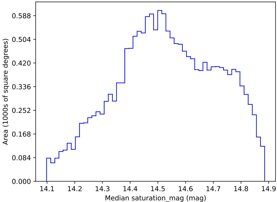
ddf_acor_sf10_lsf30_lsr10_v3.4_10yrs WFD i band: Median saturation_mag
