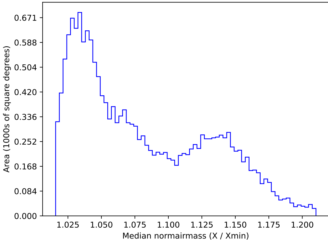
ddf_acor_sf10_lsf30_lsr10_v3.4_10yrs WFD g band: Median normairmass
