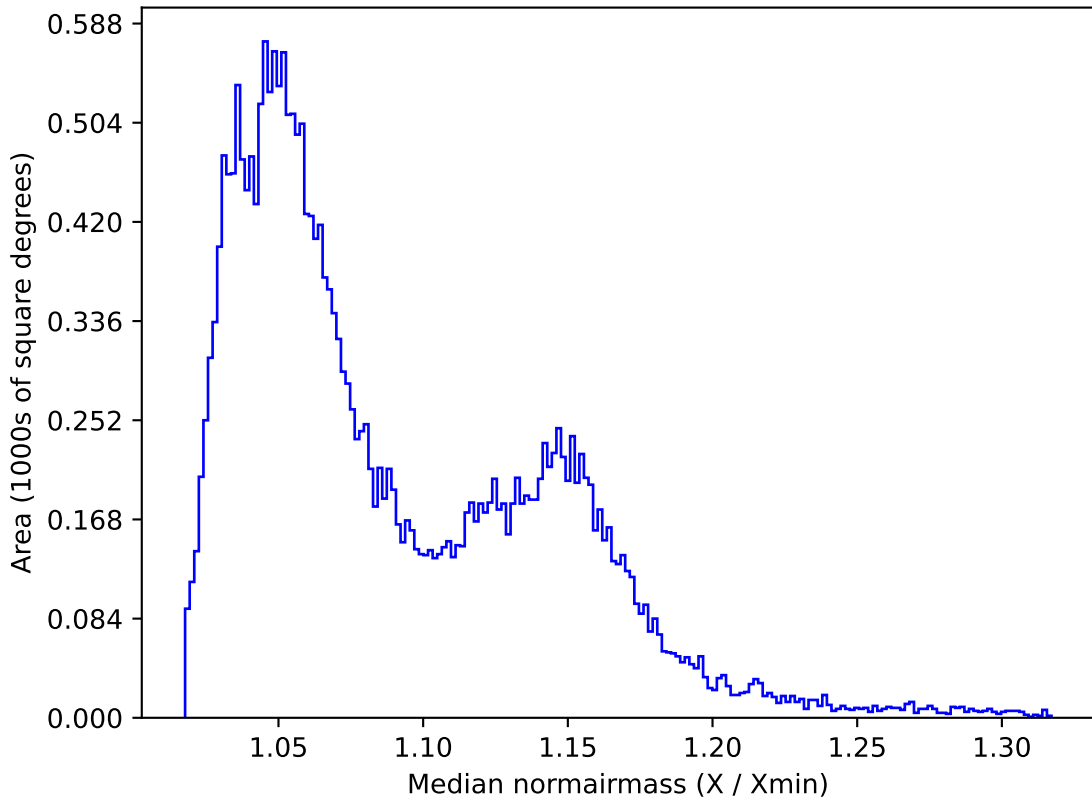
ddf_acor_sf10_lsf30_lsr10_v3.4_10yrs All sky z band: Median normairmass
