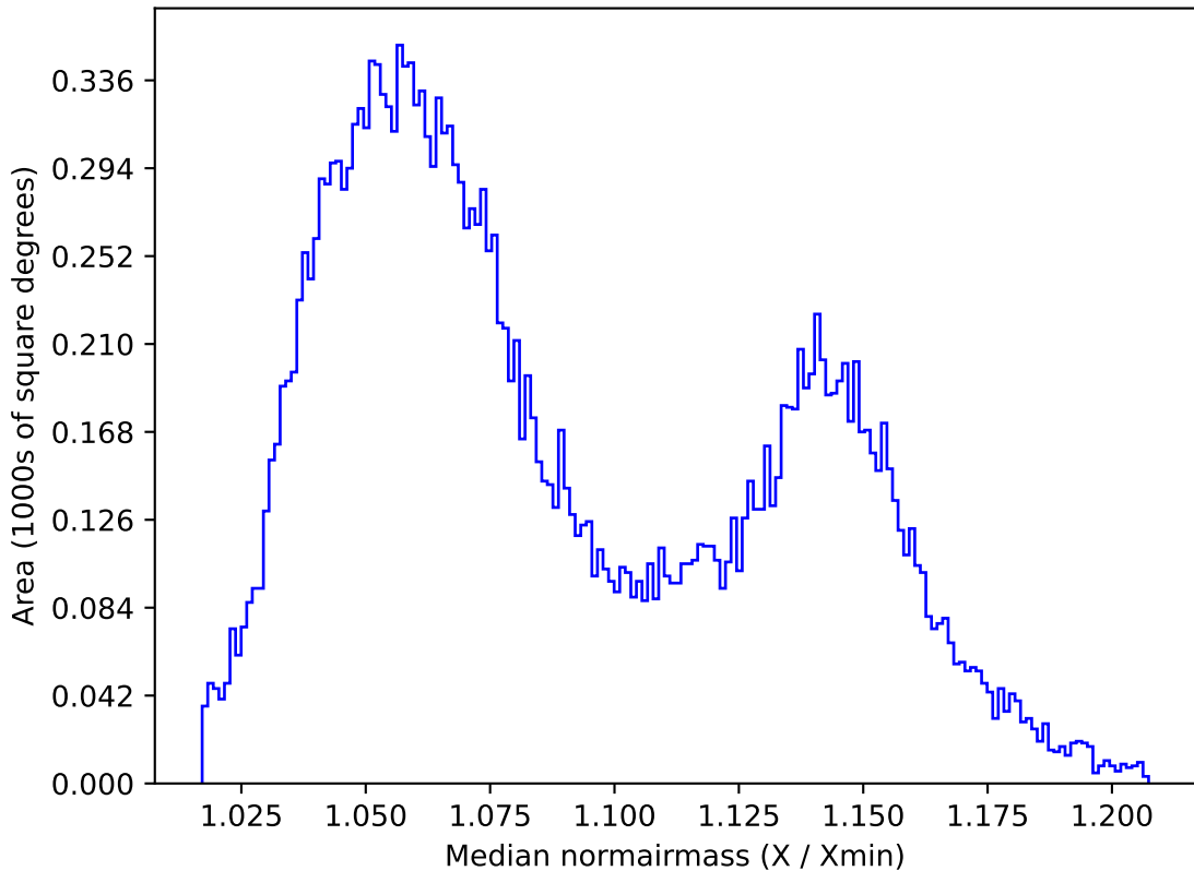
ddf_acor_sf10_lsf30_lsr10_v3.4_10yrs All sky y band: Median normairmass
