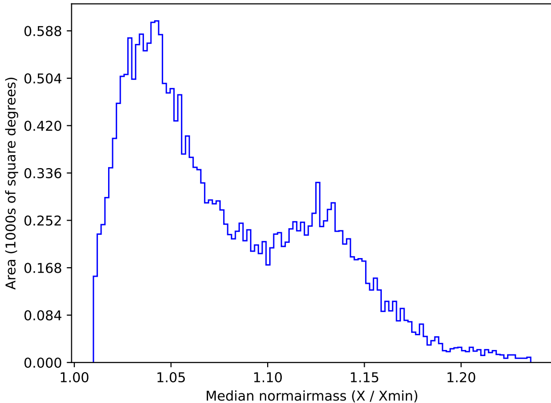
ddf_acor_sf10_ls30_lsr10_v3.4_10yrs All sky u band: Median normairmass
