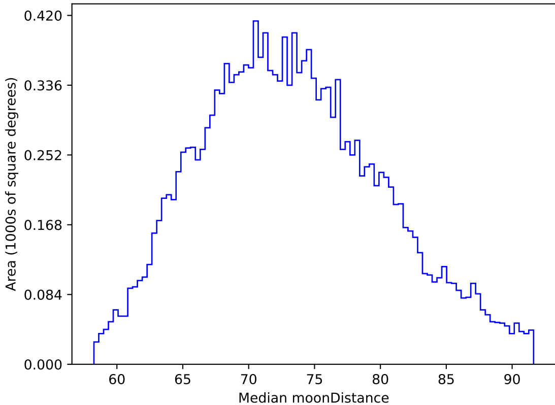
ddf_acor_sf10_lsf30_lsr10_v3.4_10yrs WFD z band: Median moonDistance
