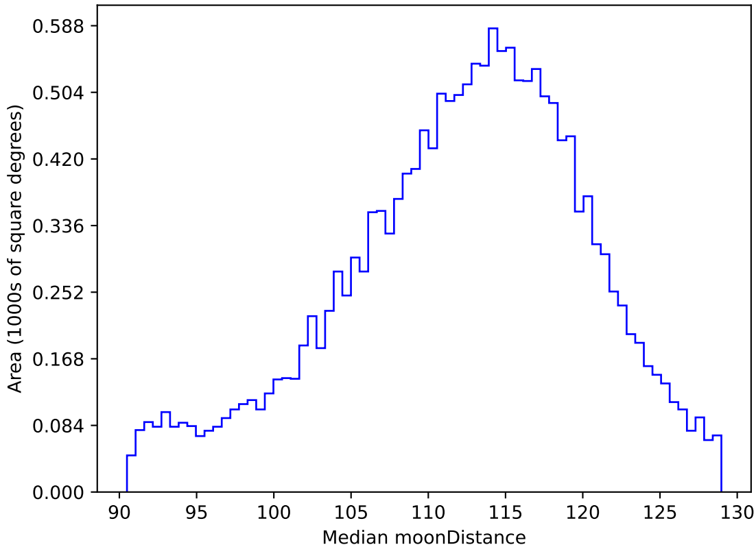
ddf_acor_sf10_lsf30_lsr10_v3.4_10yrs WFD r band: Median moonDistance
