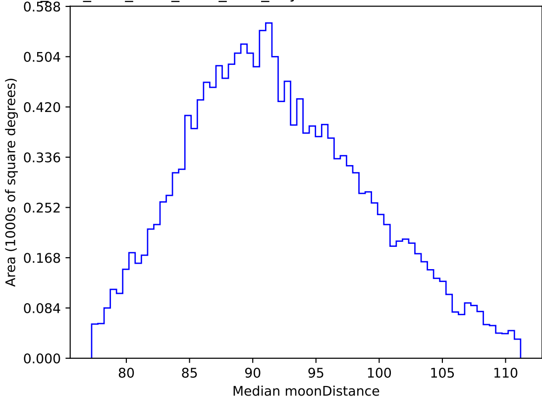
ddf_acor_sf10_lsf30_lsr10_v3.4_10yrs WFD i band: Median moonDistance
