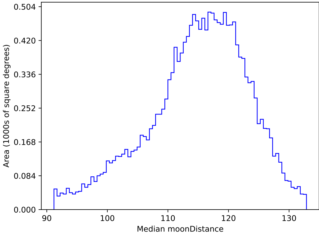
ddf_acor_sf10_lsf30_lsr10_v3.4_10yrs WFD g band: Median moonDistance
