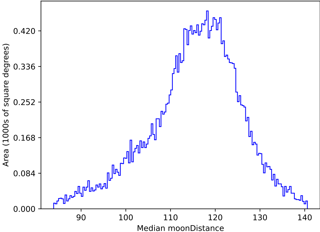
ddf_acor_sf10_lsf30_lsr10_v3.4_10yrs All sky g band: Median moonDistance
