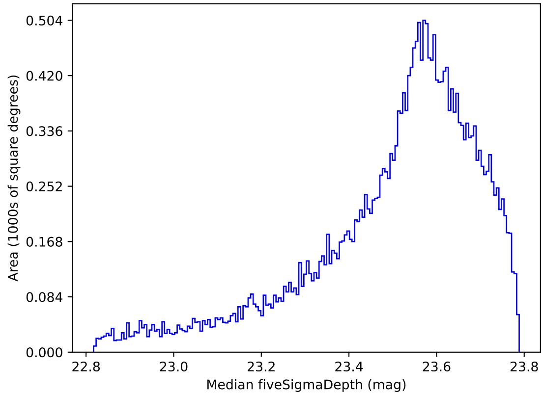
ddf_acor_sf10_lsf30_lsr10_v3.4_10yrs All sky i band: Median fiveSigmaDepth
