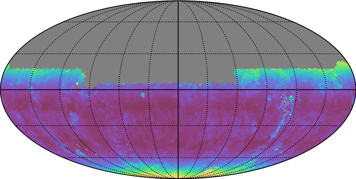
ddf_acor_sf10_lsf30_lsr10_v3.4_10yrs Yr 1 y band: Median airmass
