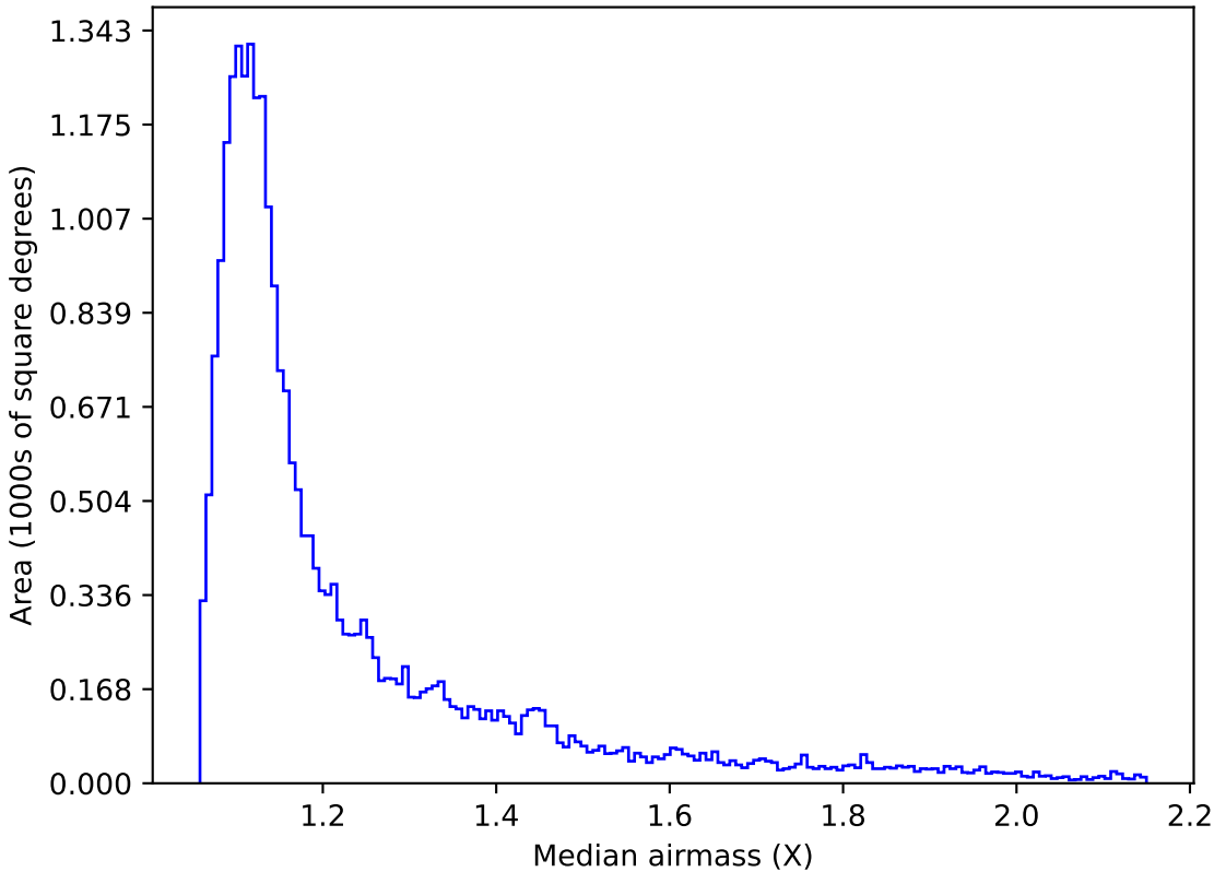
ddf_acor_sf10_lsf30_lsr10_v3.4_10yrs Yr 1 i band: Median airmass
