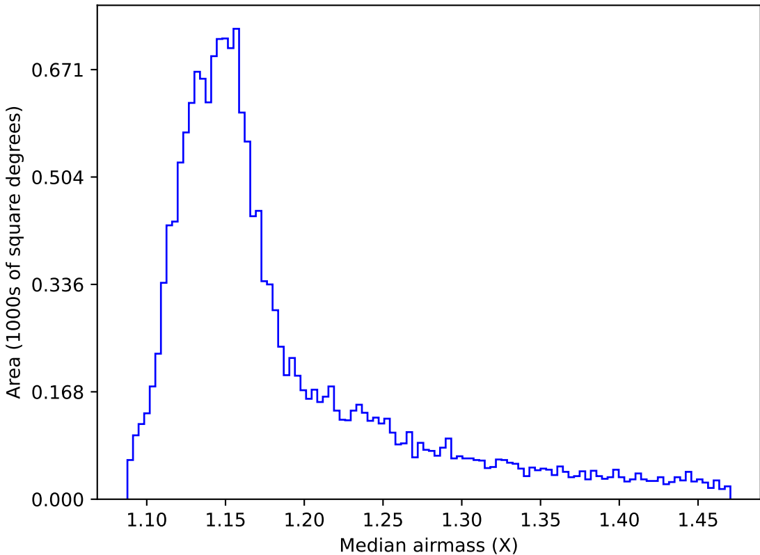
ddf_acor_sf10_lsf30_lsr10_v3.4_10yrs WFD z band: Median airmass
