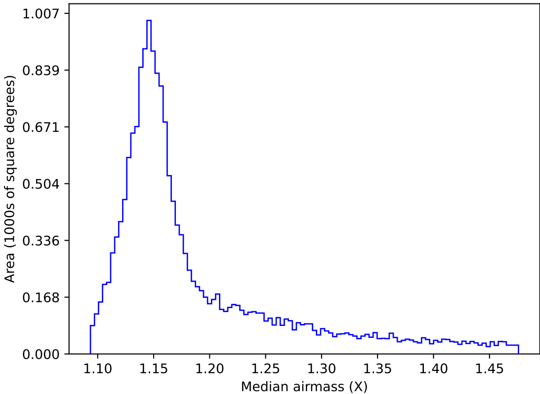
ddf_acor_sf10_lsf30_lsr10_v3.4_10yrs WFD y band: Median airmass
