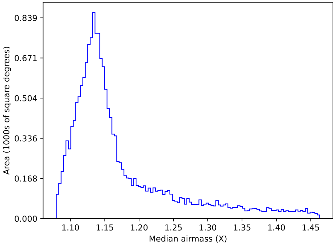
ddf_acor_sf10_lsf30_lsr10_v3.4_10yrs WFD i band: Median airmass
