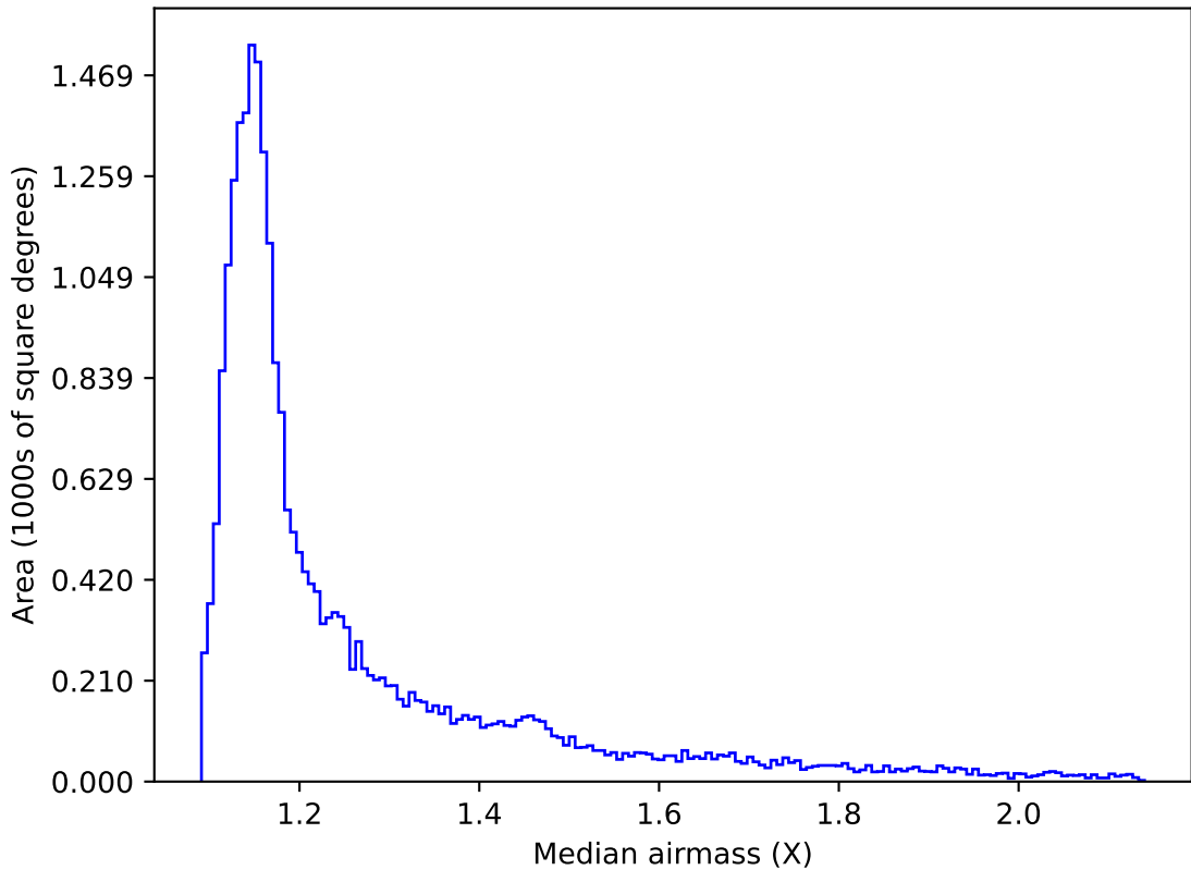
ddf_acor_sf10_lsf30_lsr10_v3.4_10yrs All sky z band: Median airmass
