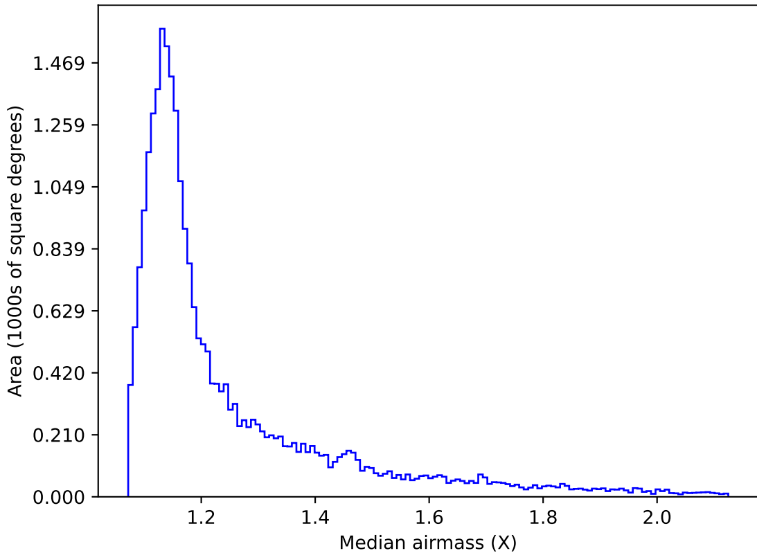
ddf_acor_sf10_lsf30_lsr10_v3.4_10yrs All sky g band: Median airmass
