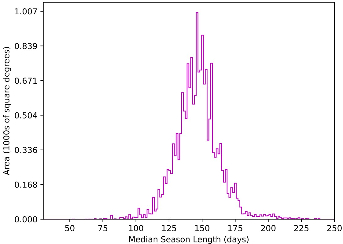
ddf_acor_sf10_lsf30_lsr10_v3.4_10yrs WFD z band: Median Season Length
