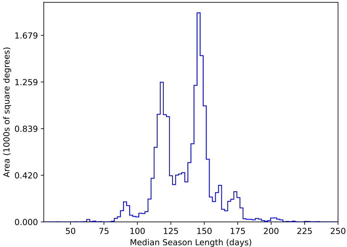
ddf_acor_sf10_lsf30_lsr10_v3.4_10yrs WFD y band: Median Season Length
