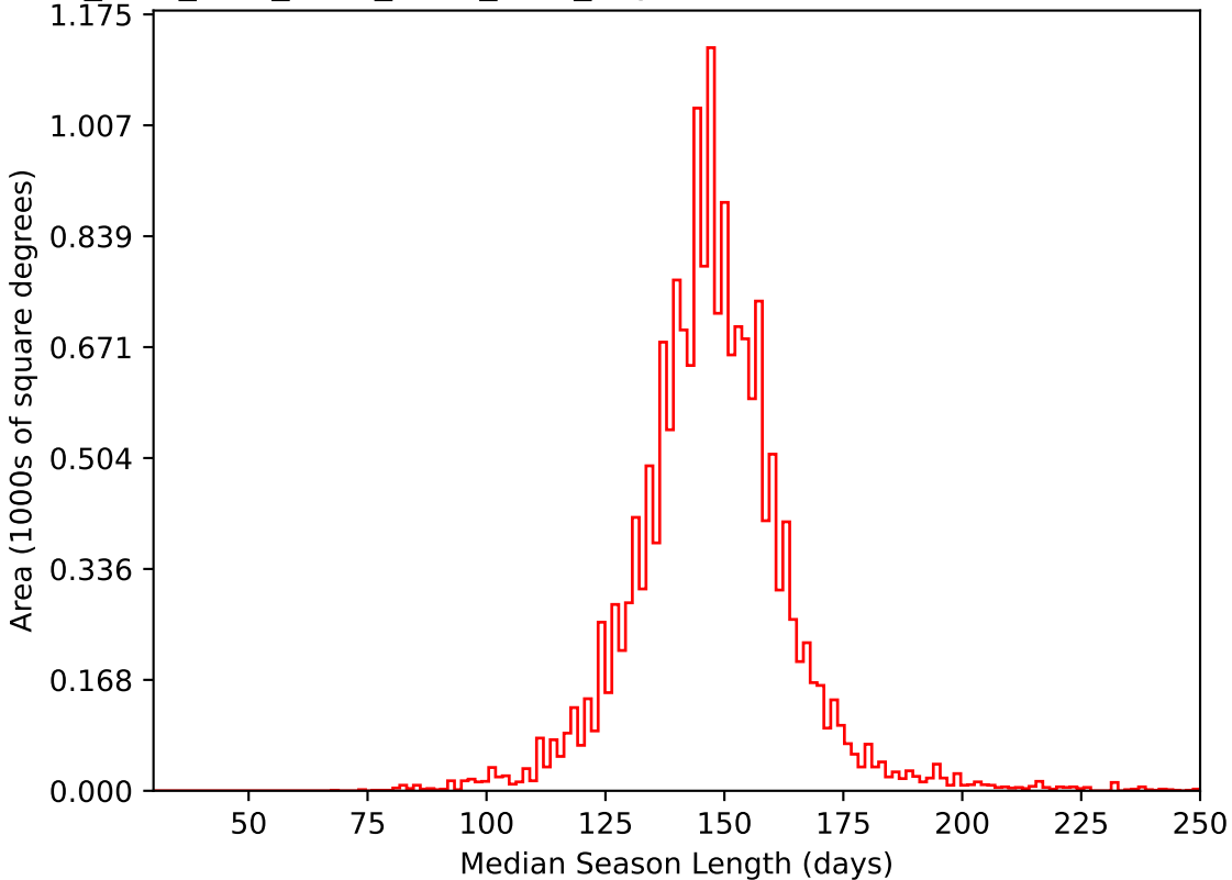
ddf_acor_sf10_lsf30_lsr10_v3.4_10yrs WFD i band: Median Season Length
