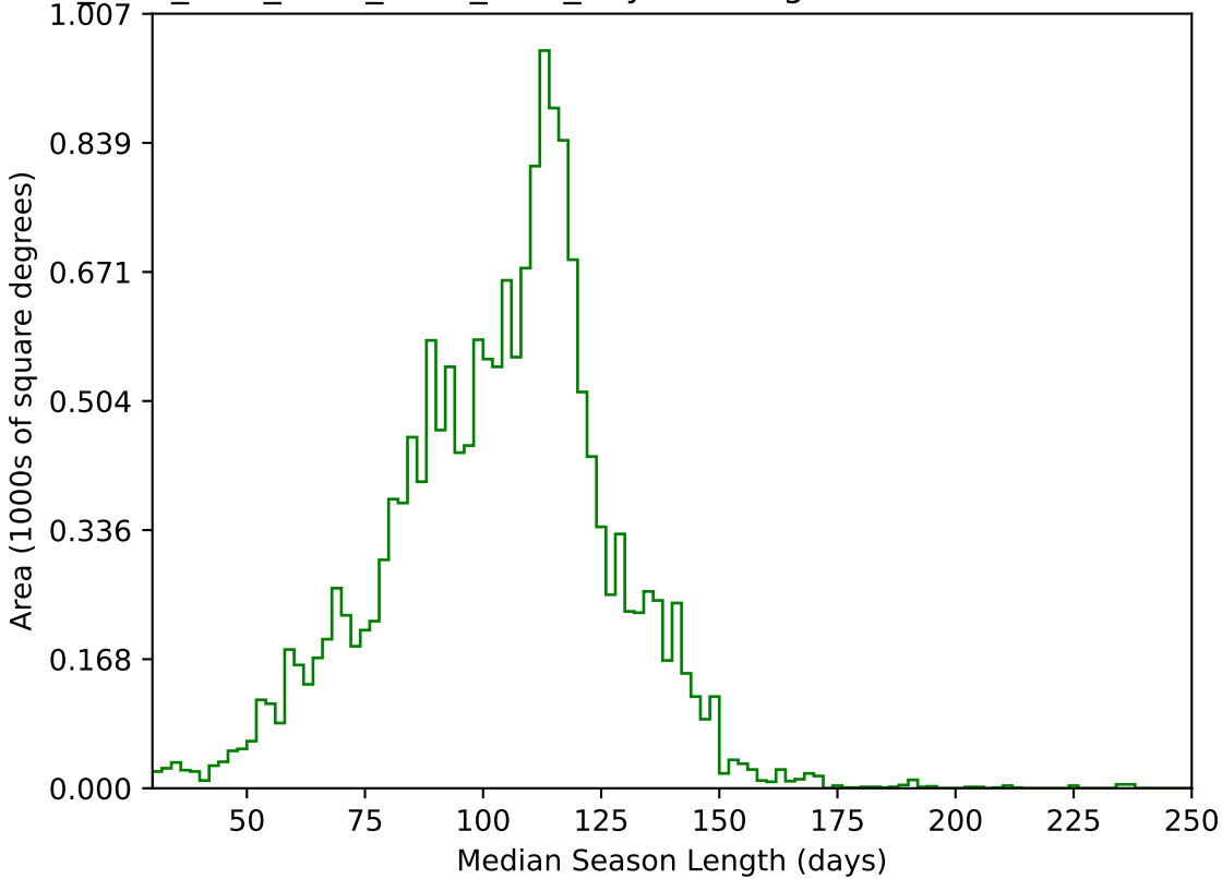
ddf_acor_sf10_ls30_lsr10_v3.4_10yrs WFD g band: Median Season Length
