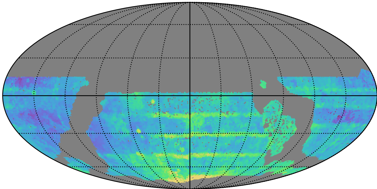
ddf_acor_sf10_lsf30_lsr10_v3.4_10yrs WFD all bands: Median Season Length
