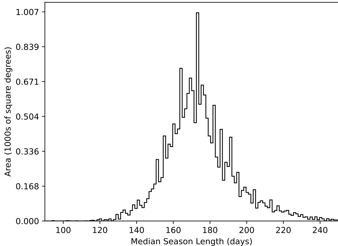
ddf_acor_sf10_lsf30_lsr10_v3.4_10yrs WFD all bands: Median Season Length
