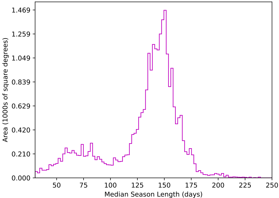
ddf_acor_sf10_lsf30_lsr10_v3.4_10yrs All sky z band: Median Season Length
