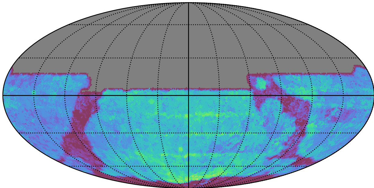
ddf_acor_sf10_lsf30_lsr10_v3.4_10yrs All sky y band: Median Season Length
